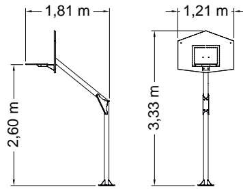
CANASTA MINIBASKET Ref. 80926
